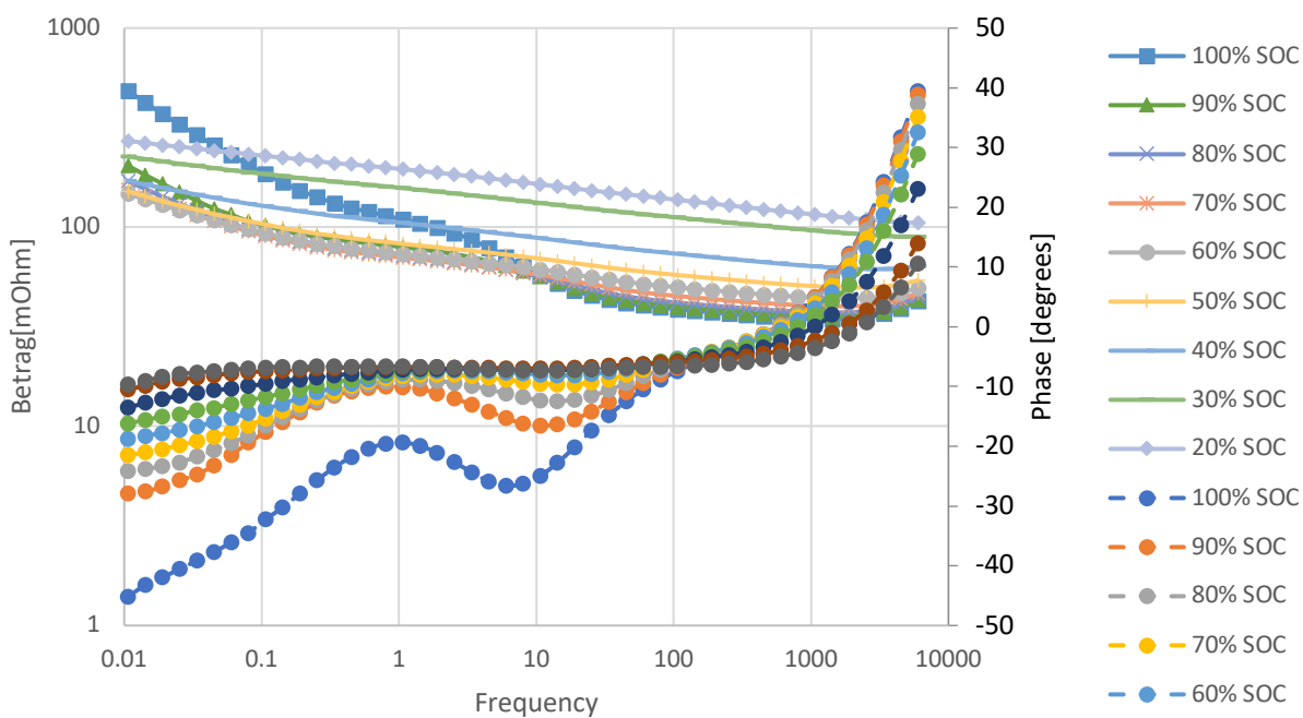
Frequency response of small signal impedance at different SOC (Solid line - Magnitude of impedance , dashed line - Phase angle)
